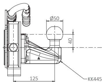
Maße mit/ Dimensions with KK445
