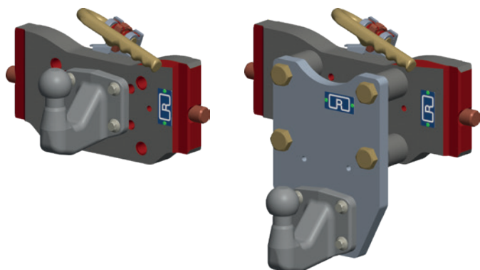
Maße mit/ Dimensions with KK445
